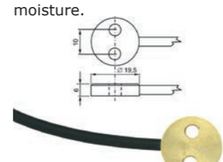
Pt1000TG7/E (-30°C to +200°C)
